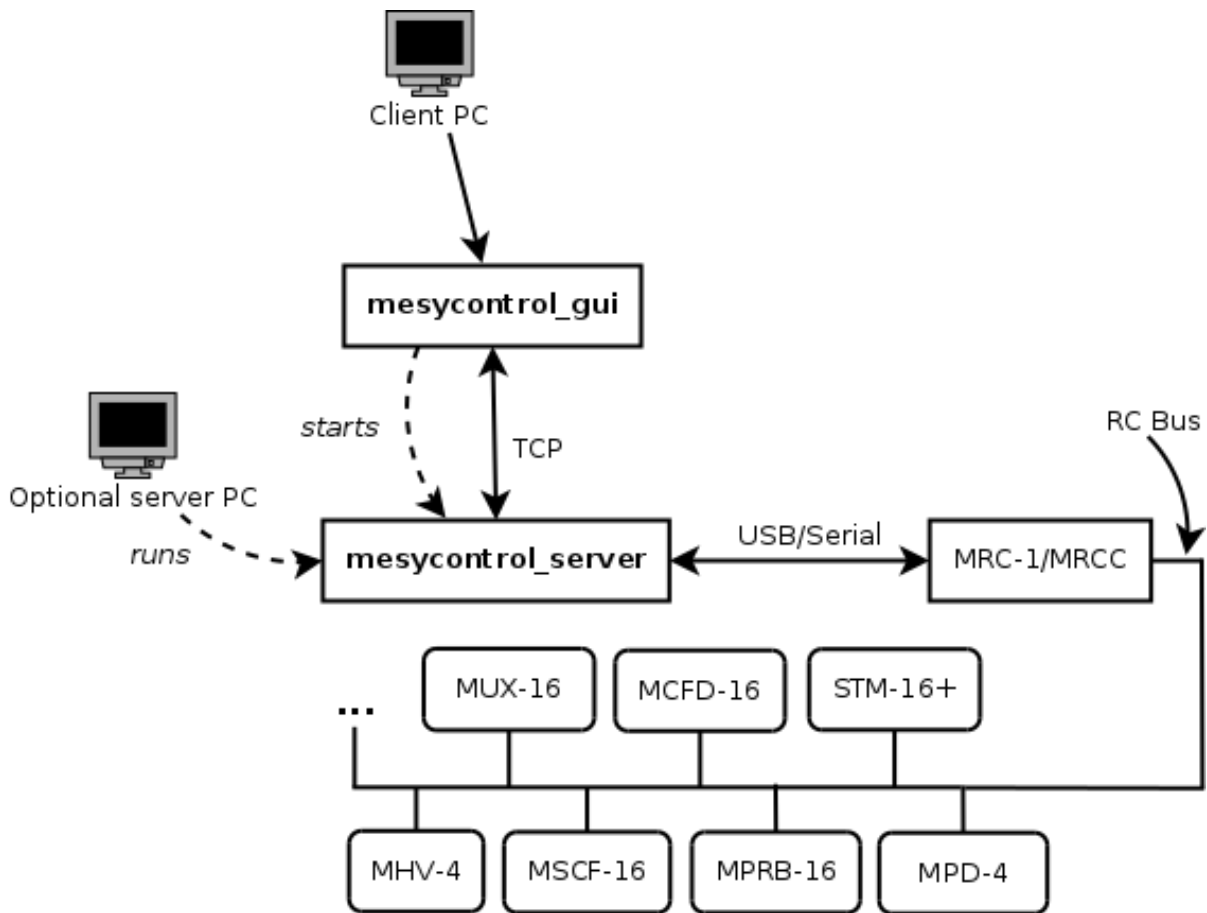
Fig. 1: mesycontrol architecture
